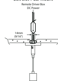
T2 - 14mm (9/16") Bolt Slot T-Bar Mount
